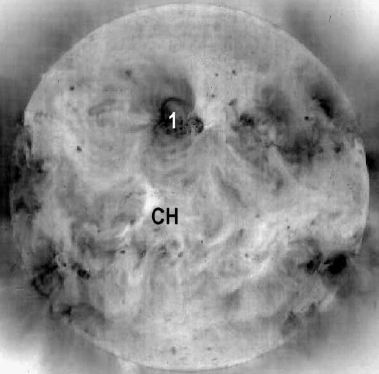
c SOHO/EIT, 284 A
