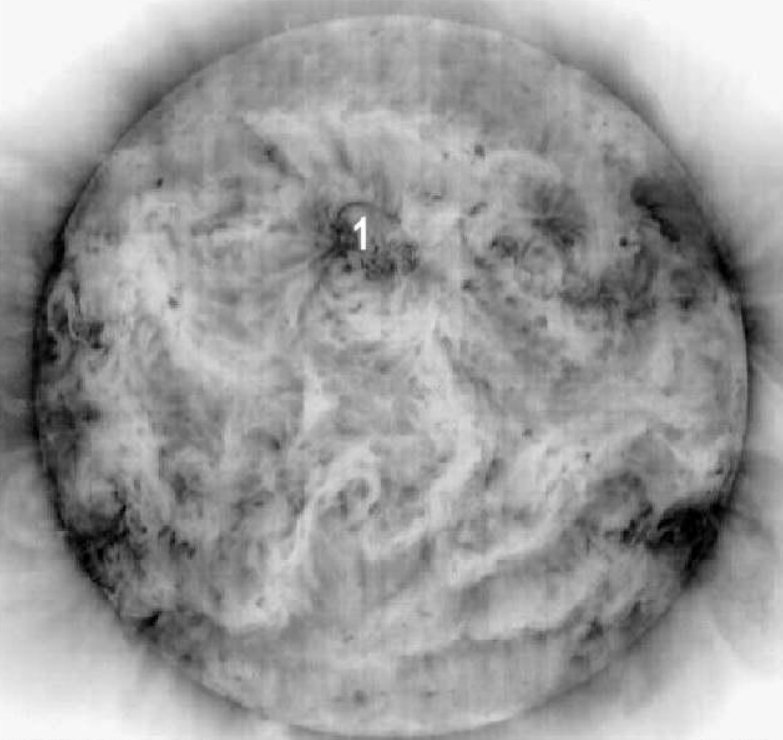
b SOHO/EIT, 195 A
