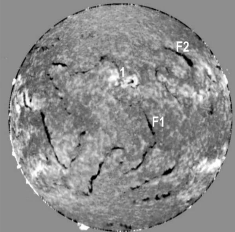
a Paris Obs., H-alpha
